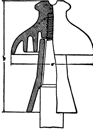
FIG. 8. MISSOURI-RIVER INSULATOR.
